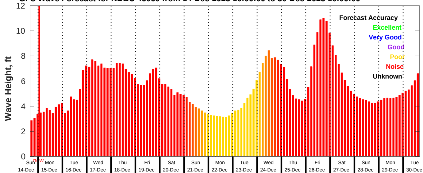
GFS Wave Forecast for NDBC 46069 from 14-Dec-2025 16:00:00 to 30-Dec-2025 16:00:00
