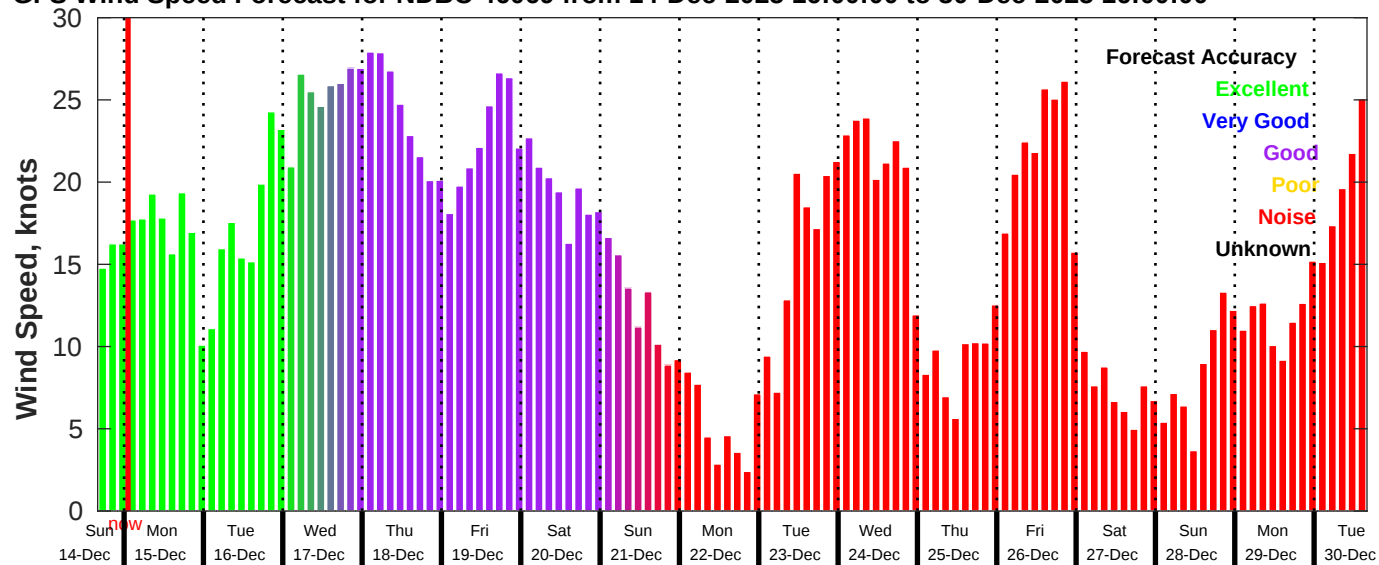
GFS Wind Speed Forecast for NDBC 46069 from 14-Dec-2025 16:00:00 to 30-Dec-2025 16:00:00
