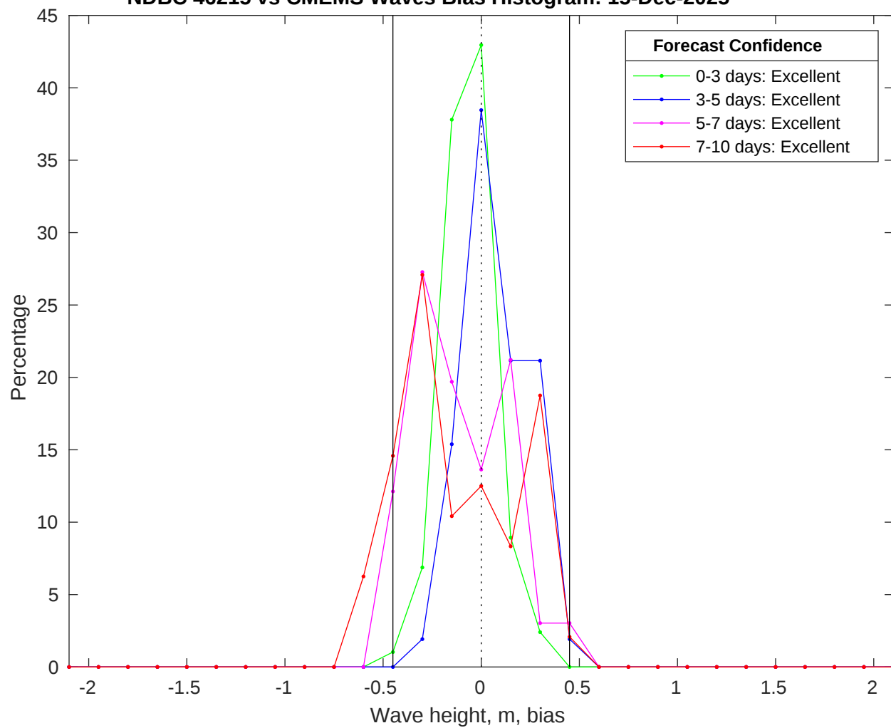
NDBC 46215 vs CMEMS Waves Bias Histogram: 15-Dec-2025
