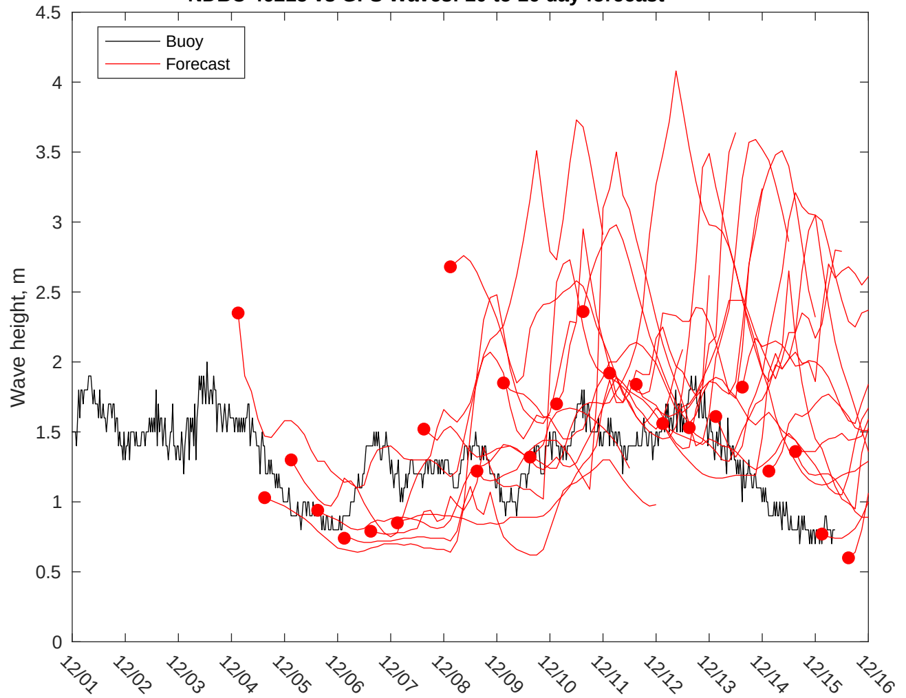
NDBC 46215 vs GFS Waves: 10 to 16 day forecast
