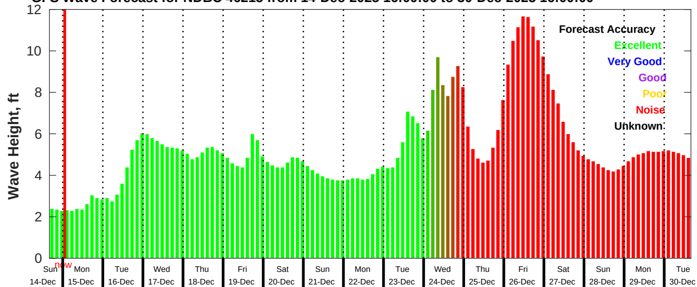
GFS Wave Forecast for NDBC 46215 from 14-Dec-2025 16:00:00 to 30-Dec-2025 16:00:00
