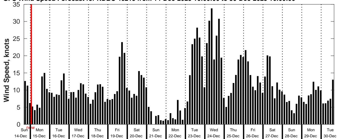
GFS Wind Speed Forecast for NDBC 46215 from 14-Dec-2025 16:00:00 to 30-Dec-2025 16:00:00
