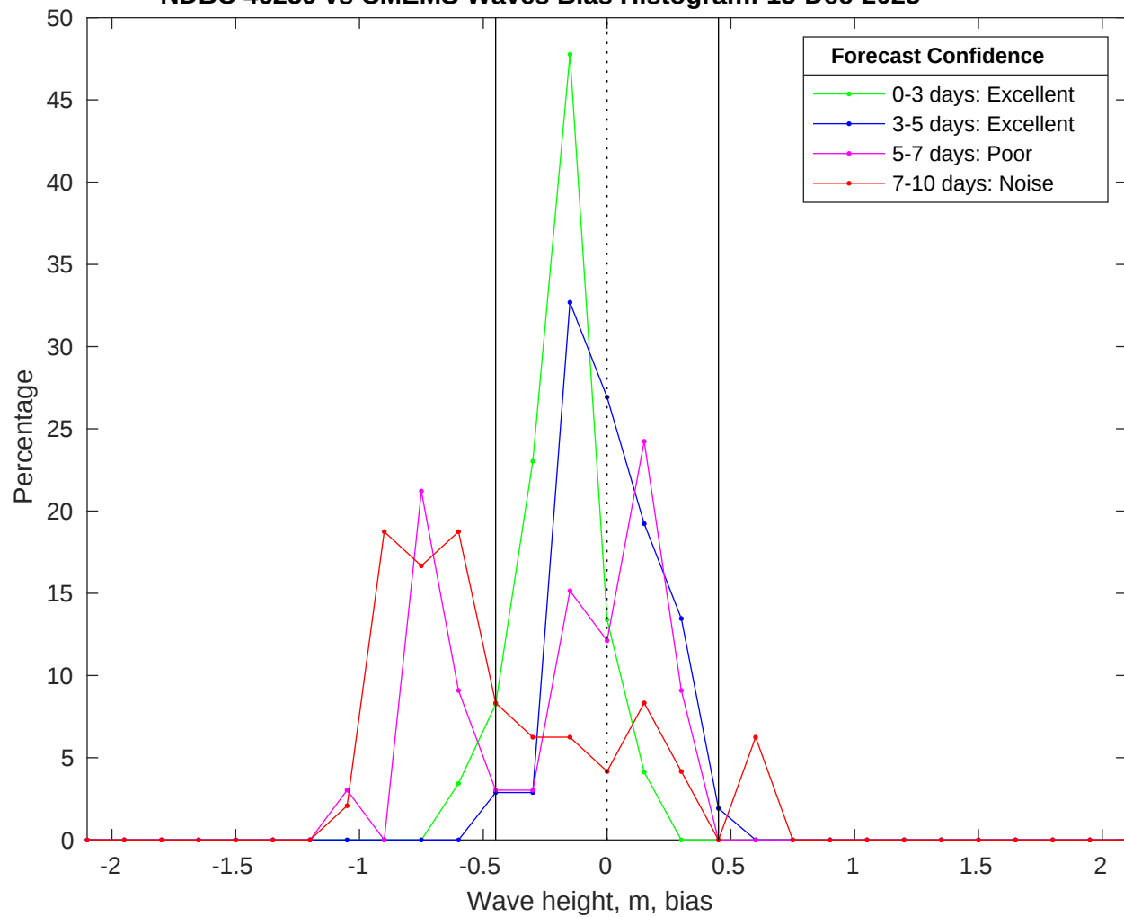
NDBC 46259 vs CMEMS Waves Bias Histogram: 15-Dec-2025
