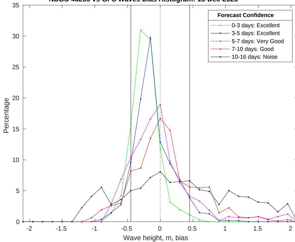
NDBC 46259 vs GFS Waves Bias Histogram: 15-Dec-2025
