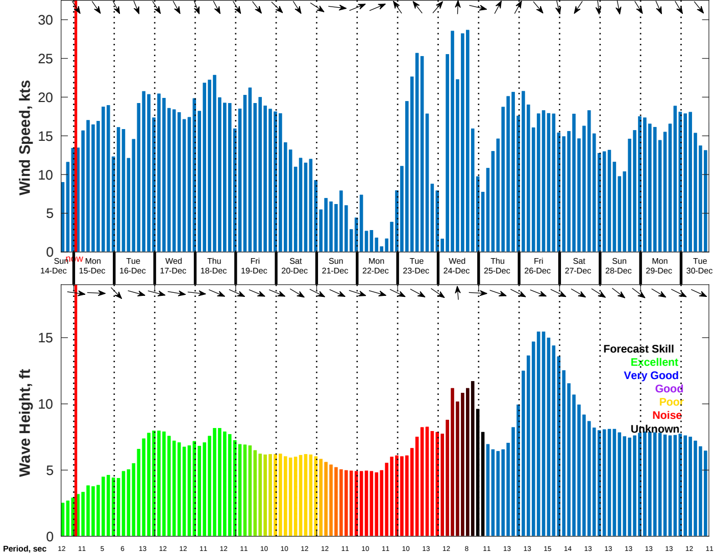
Wind & Wave Forecast for NDBC 46259 from 14-Dec-2025 16:00:00 to 30-Dec-2025 16:00:00
