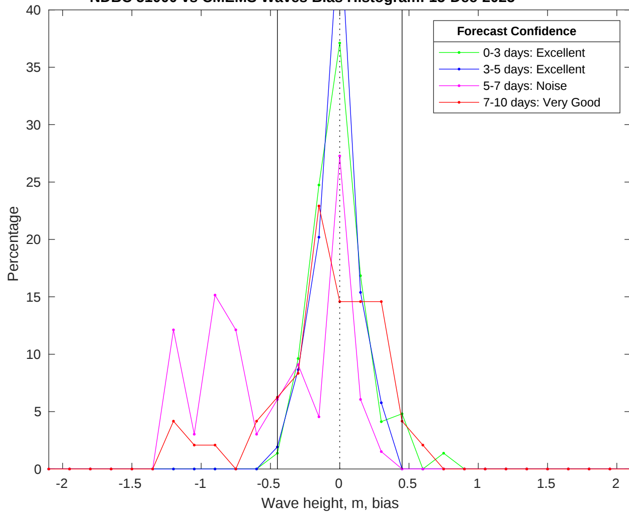
NDBC 51000 vs CMEMS Waves Bias Histogram: 15-Dec-2025
