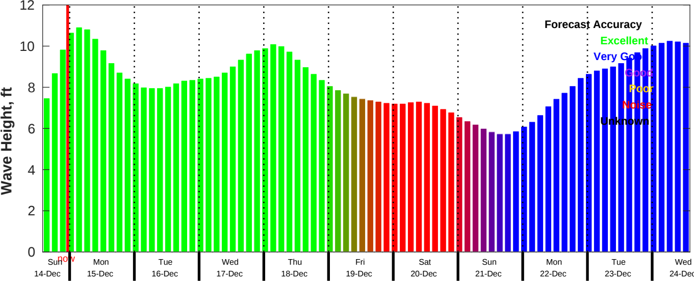
CMEMS Wave Forecast for NDBC 51000 from 14-Dec-2025 14:00:00 to 24-Dec-2025 14:00:00
