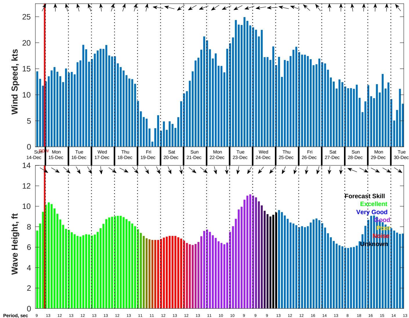
Wind & Wave Forecast for NDBC 51000 from 14-Dec-2025 14:00:00 to 30-Dec-2025 14:00:00
