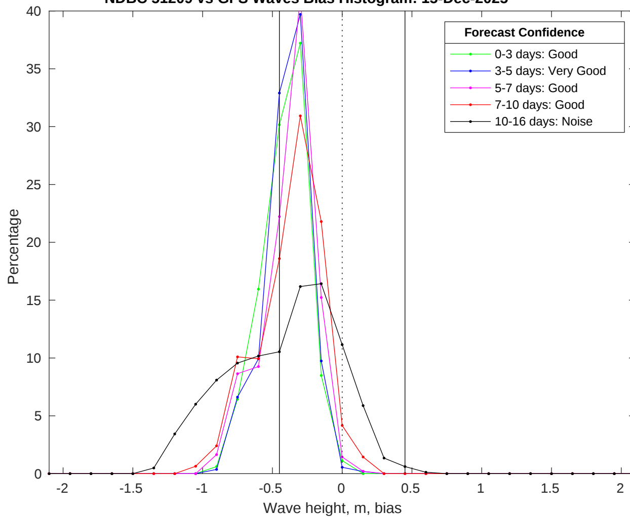
NDBC 51209 vs GFS Waves Bias Histogram: 15-Dec-2025
