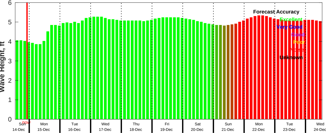
CMEMS Wave Forecast for NDBC 51209 from 14-Dec-2025 13:00:00 to 24-Dec-2025 13:00:00
