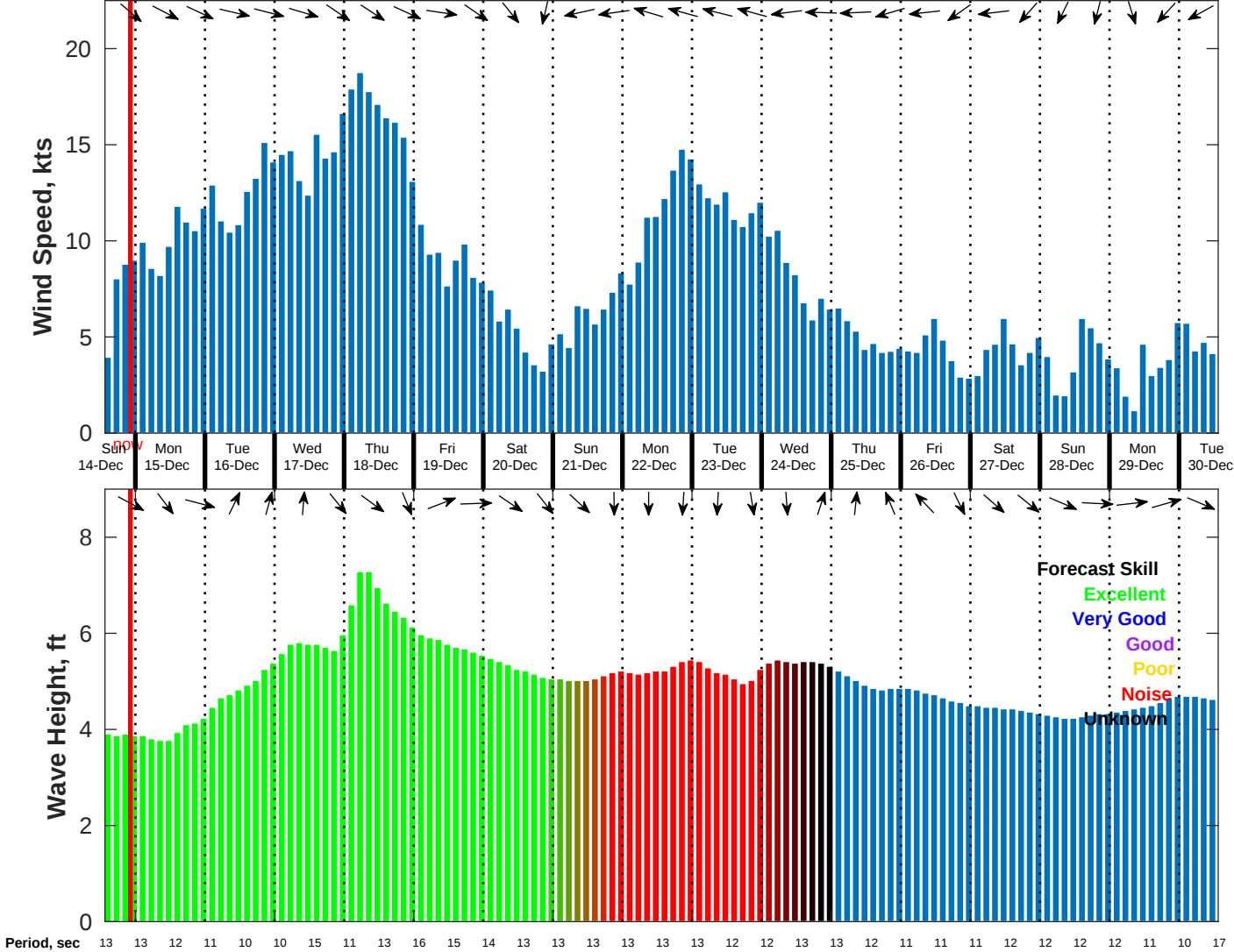
Wind & Wave Forecast for NDBC 51209 from 14-Dec-2025 13:00:00 to 30-Dec-2025 13:00:00
