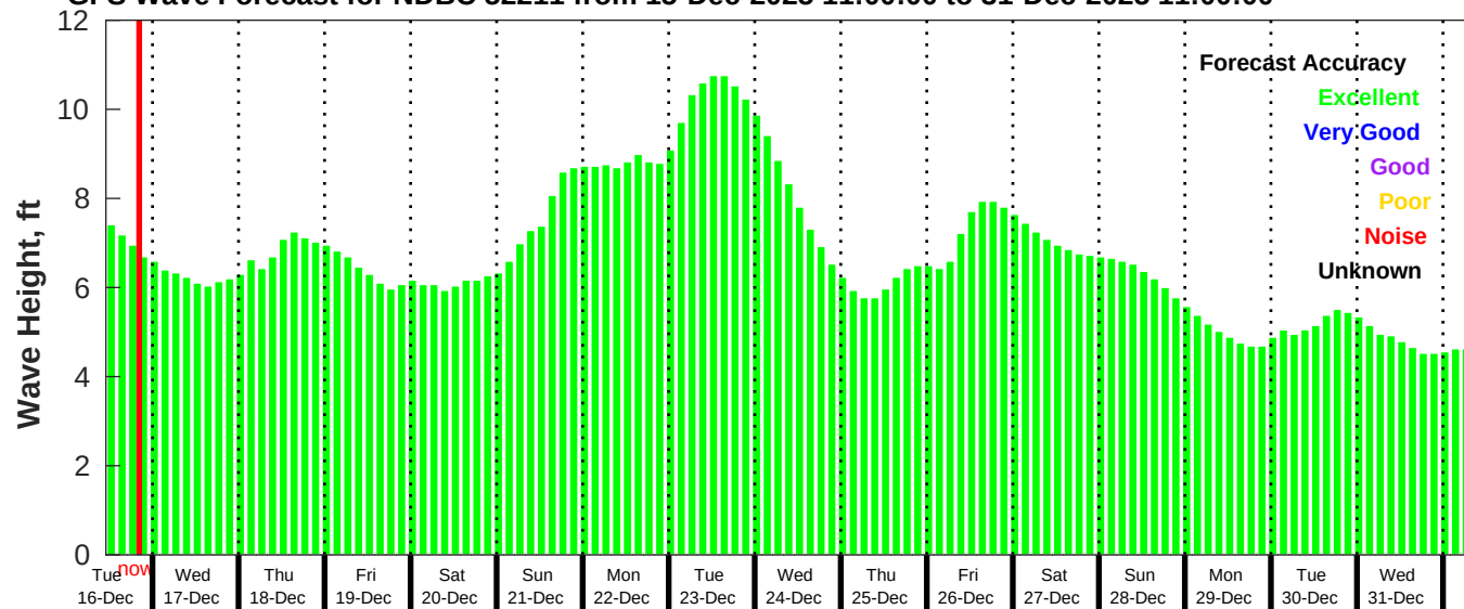
GFS Wave Forecast for NDBC 52211 from 15-Dec-2025 11:00:00 to 31-Dec-2025 11:00:00
