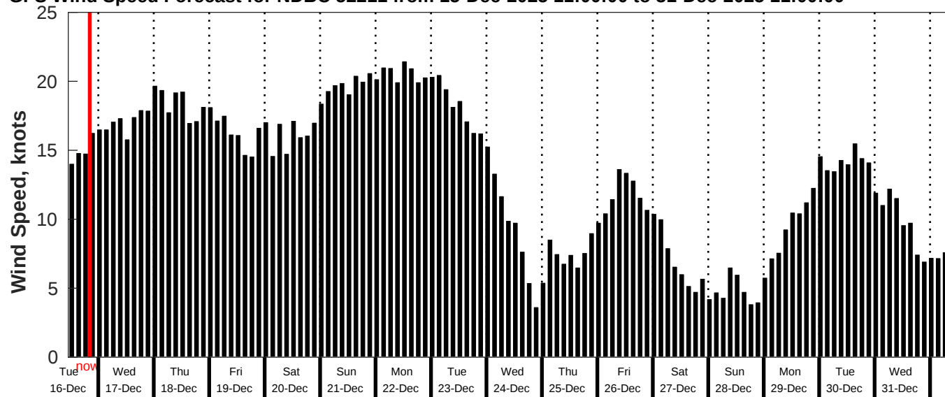
GFS Wind Speed Forecast for NDBC 52211 from 15-Dec-2025 11:00:00 to 31-Dec-2025 11:00:00
