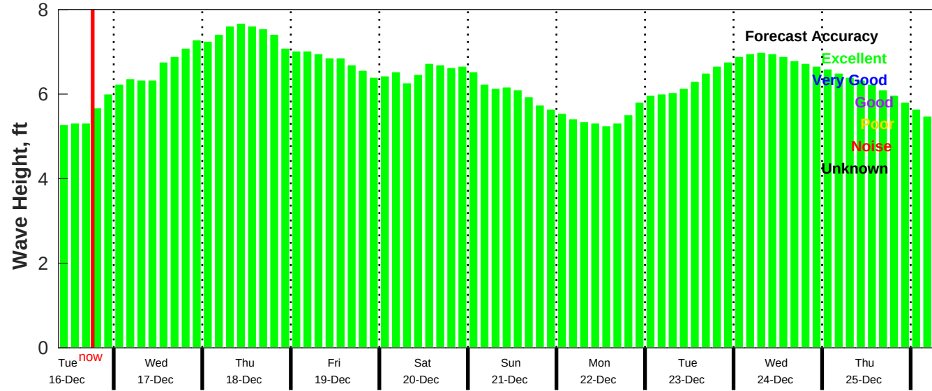
CMEMS Wave Forecast for NDBC 52212 from 15-Dec-2025 09:00:00 to 25-Dec-2025 09:00:00
