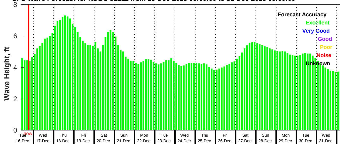
GFS Wave Forecast for NDBC 52212 from 15-Dec-2025 09:00:00 to 31-Dec-2025 09:00:00
