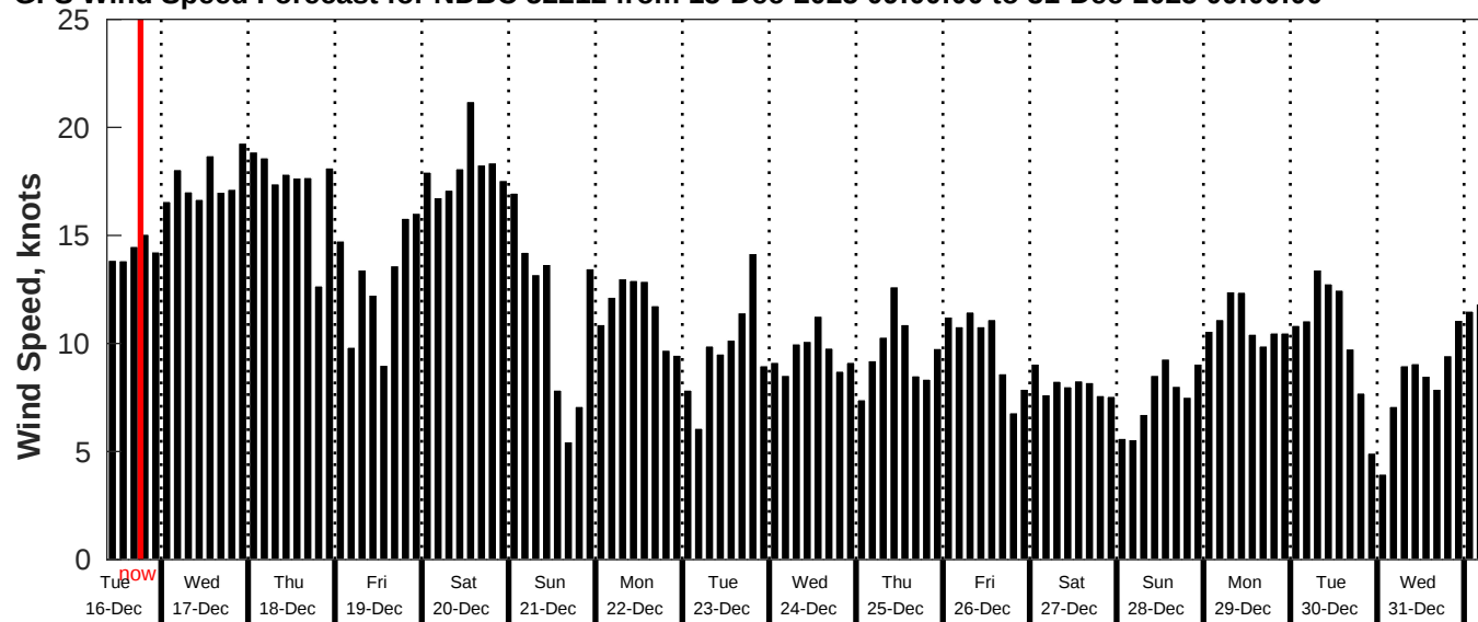
GFS Wind Speed Forecast for NDBC 52212 from 15-Dec-2025 09:00:00 to 31-Dec-2025 09:00:00
