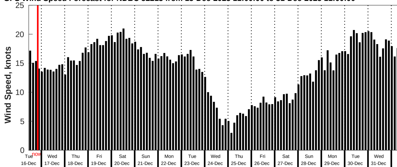
GFS Wind Speed Forecast for NDBC 52213 from 15-Dec-2025 11:00:00 to 31-Dec-2025 11:00:00
