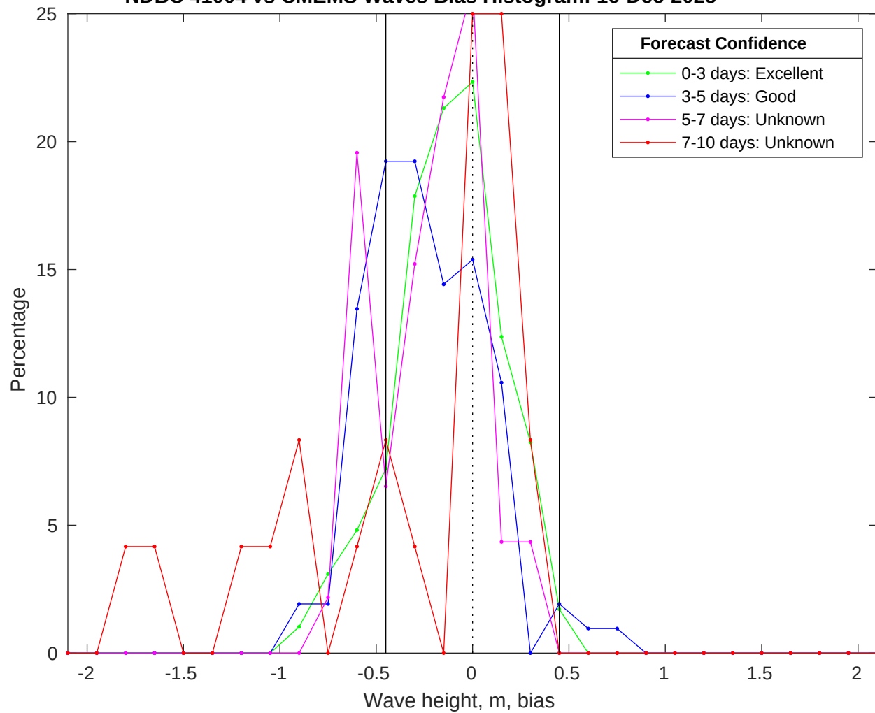
NDBC 41004 vs CMEMS Waves Bias Histogram: 16-Dec-2025
