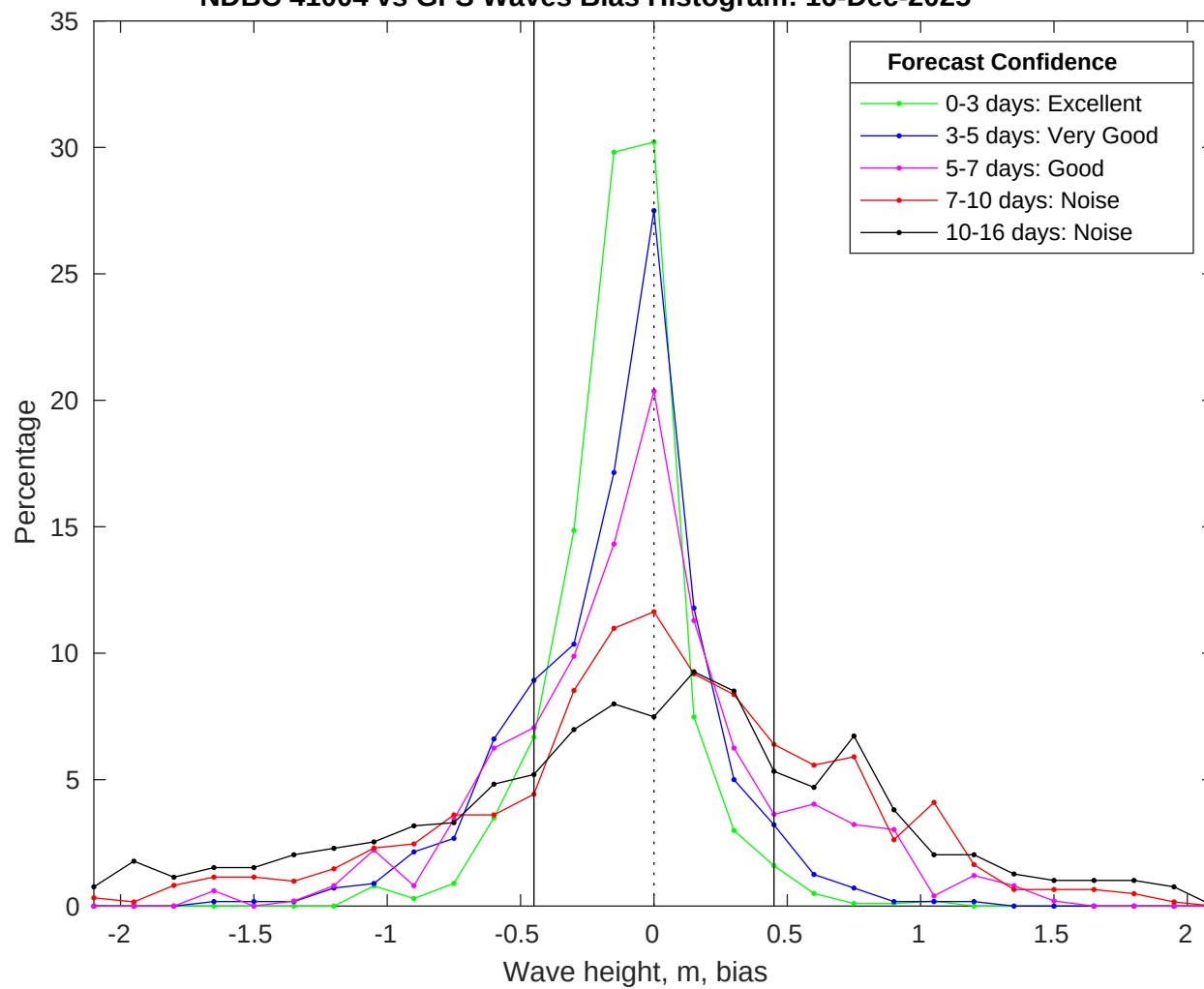
NDBC 41004 vs GFS Waves Bias Histogram: 16-Dec-2025
