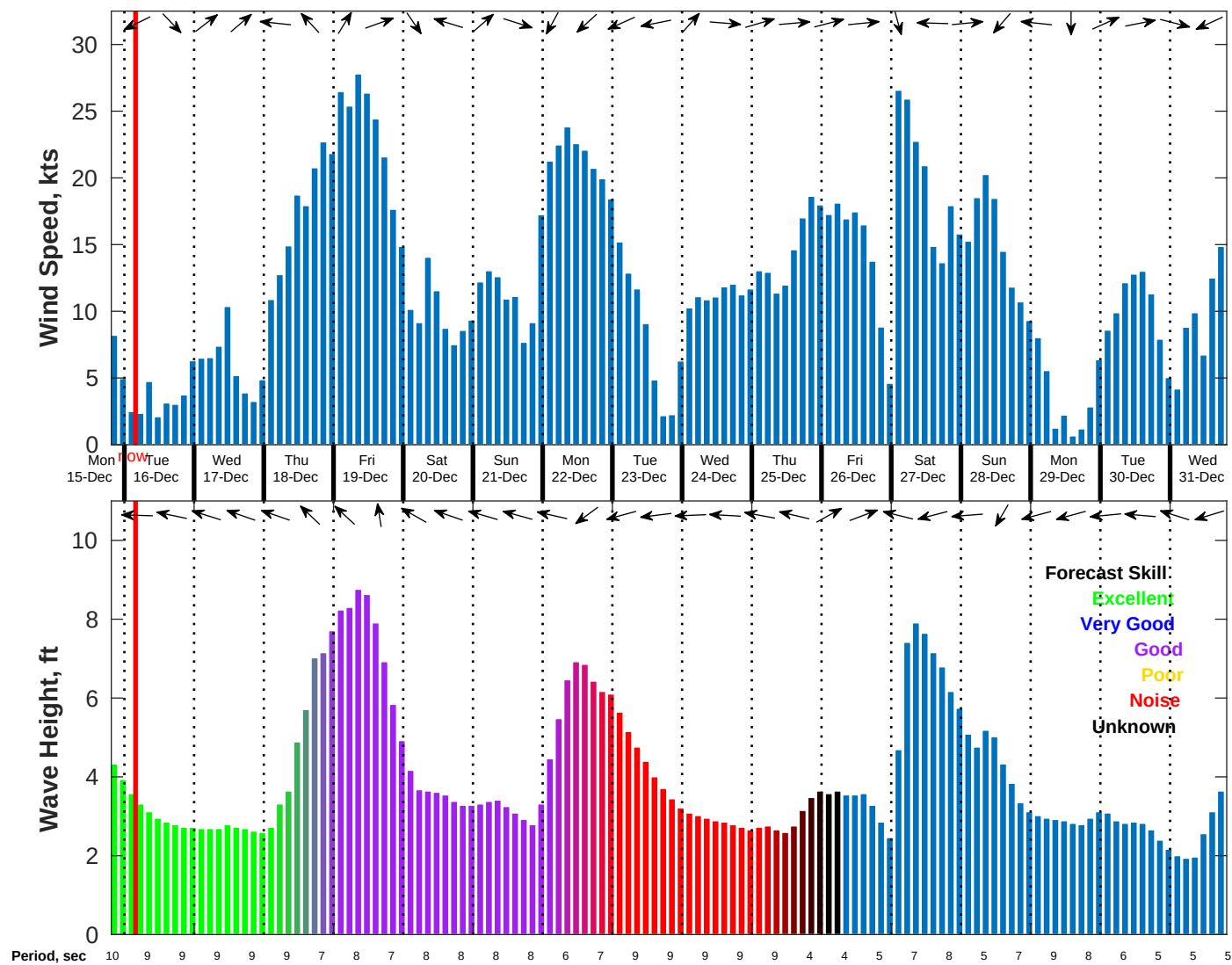
Wind & Wave Forecast for NDBC 41004 from 15-Dec-2025 19:00:00 to 31-Dec-2025 19:00:00
