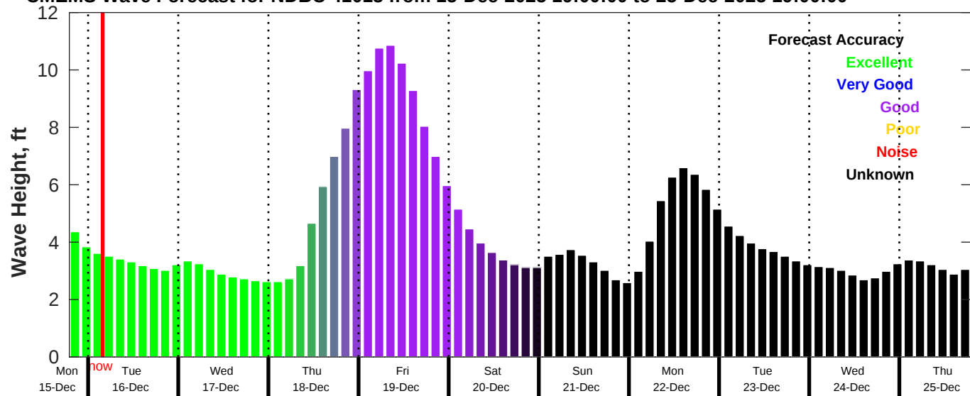
CMEMS Wave Forecast for NDBC 41013 from 15-Dec-2025 19:00:00 to 25-Dec-2025 19:00:00
