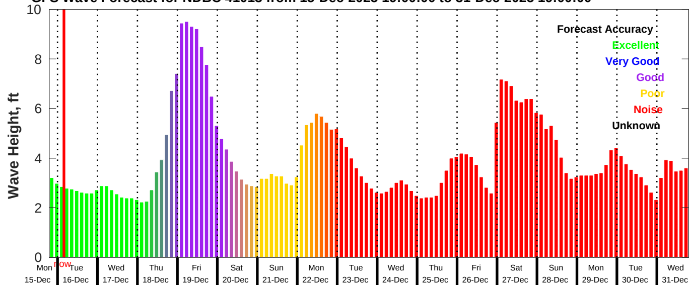
GFS Wave Forecast for NDBC 41013 from 15-Dec-2025 19:00:00 to 31-Dec-2025 19:00:00
