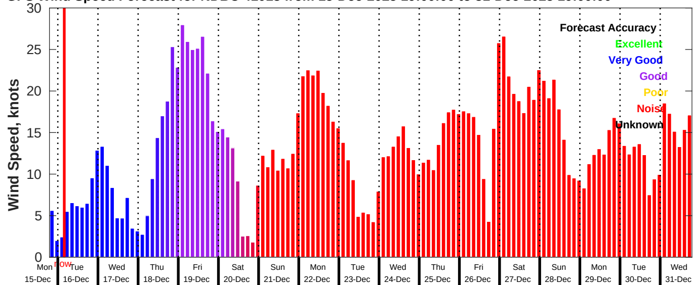
GFS Wind Speed Forecast for NDBC 41013 from 15-Dec-2025 19:00:00 to 31-Dec-2025 19:00:00
