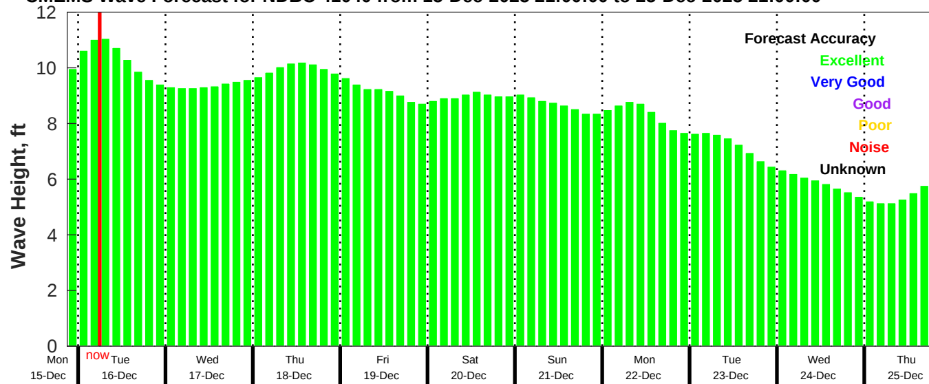
CMEMS Wave Forecast for NDBC 41040 from 15-Dec-2025 21:00:00 to 25-Dec-2025 21:00:00
