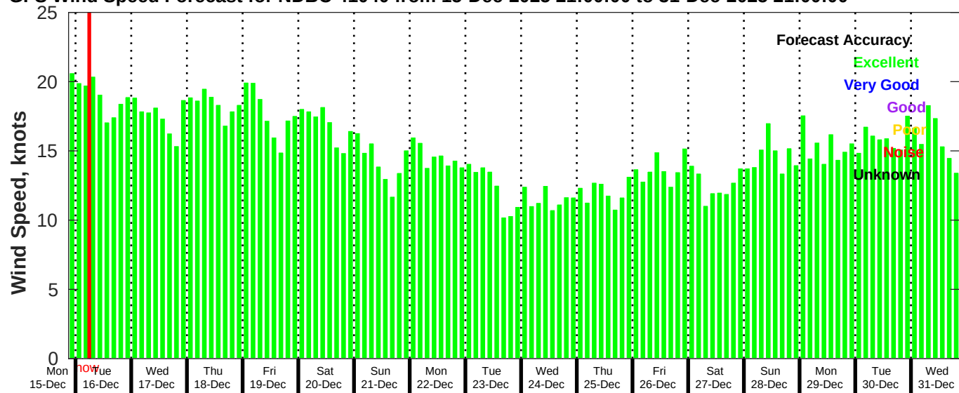
GFS Wind Speed Forecast for NDBC 41040 from 15-Dec-2025 21:00:00 to 31-Dec-2025 21:00:00
