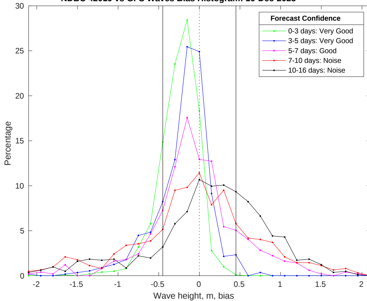
NDBC 42019 vs GFS Waves Bias Histogram: 16-Dec-2025
