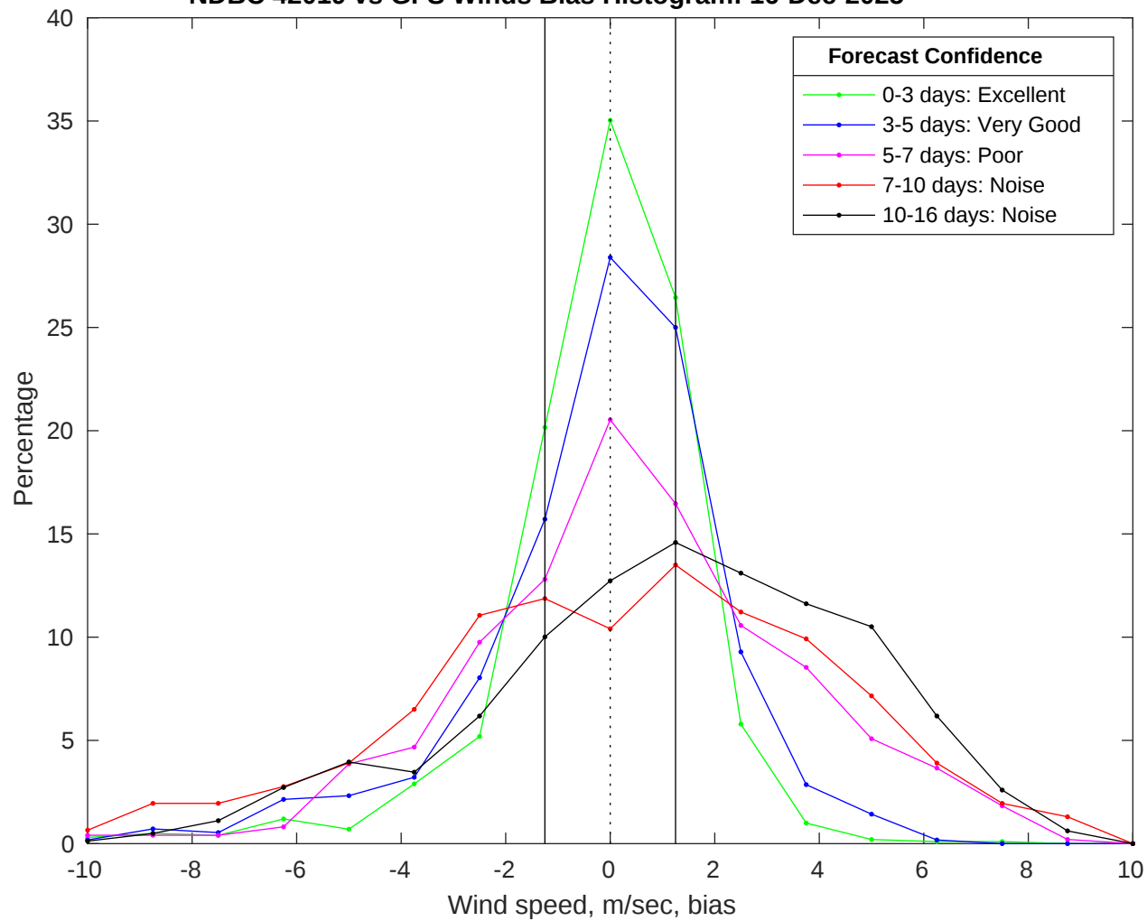
NDBC 42019 vs GFS Winds Bias Histogram: 16-Dec-2025
