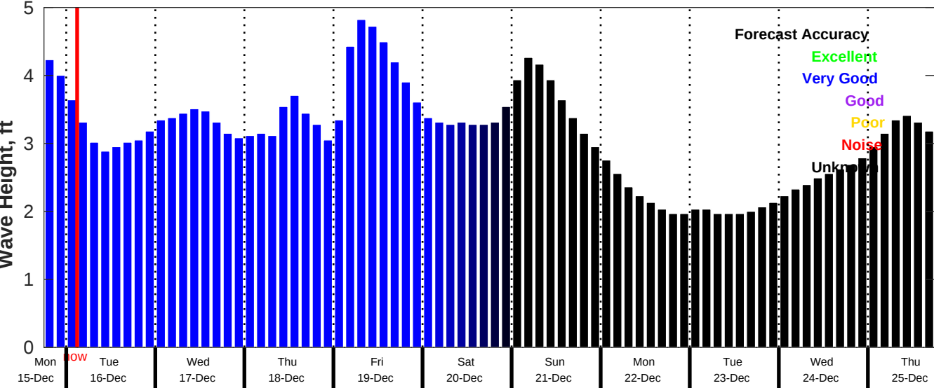
CMEMS Wave Forecast for NDBC 42019 from 15-Dec-2025 18:00:00 to 25-Dec-2025 18:00:00
