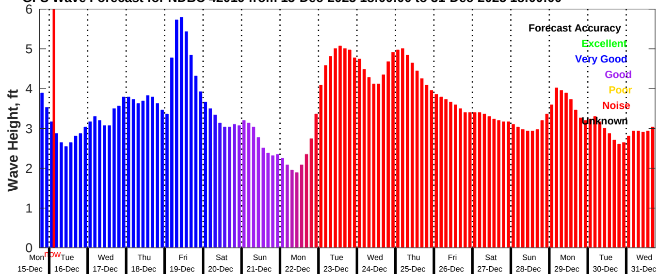
GFS Wave Forecast for NDBC 42019 from 15-Dec-2025 18:00:00 to 31-Dec-2025 18:00:00
