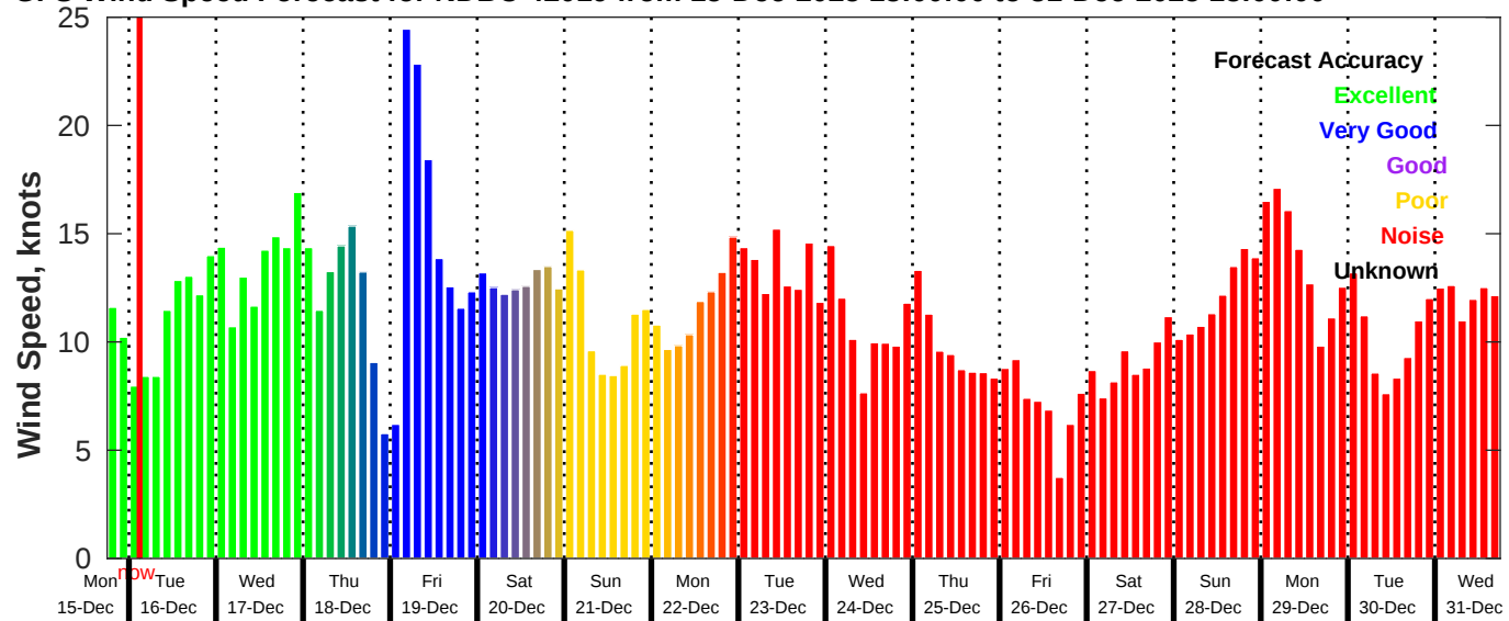
GFS Wind Speed Forecast for NDBC 42019 from 15-Dec-2025 18:00:00 to 31-Dec-2025 18:00:00
