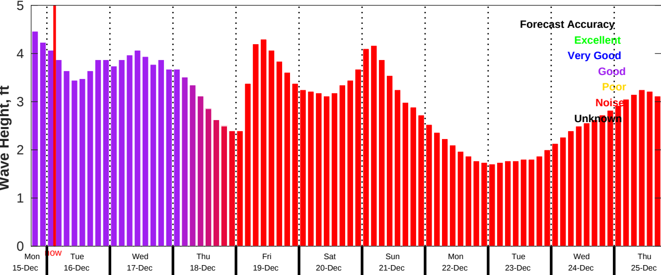
CMEMS Wave Forecast for NDBC 42020 from 15-Dec-2025 18:00:00 to 25-Dec-2025 18:00:00
