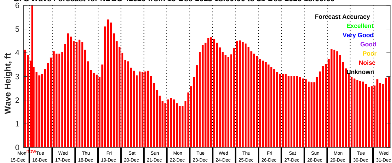
GFS Wave Forecast for NDBC 42020 from 15-Dec-2025 18:00:00 to 31-Dec-2025 18:00:00
