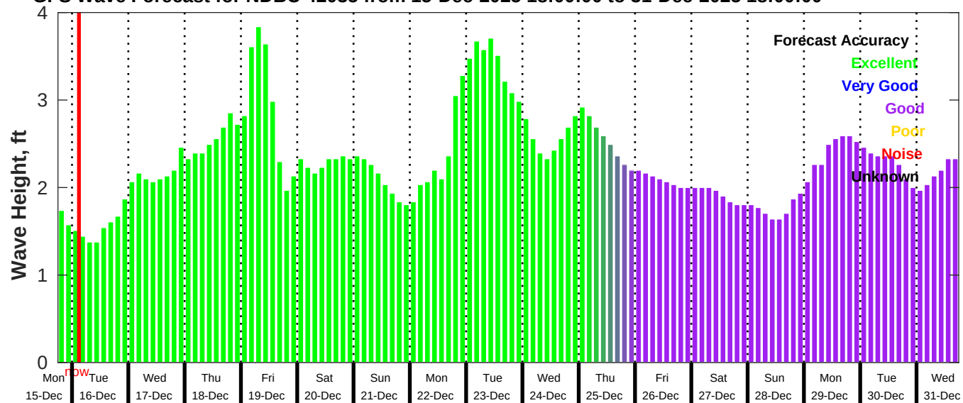
GFS Wave Forecast for NDBC 42035 from 15-Dec-2025 18:00:00 to 31-Dec-2025 18:00:00
