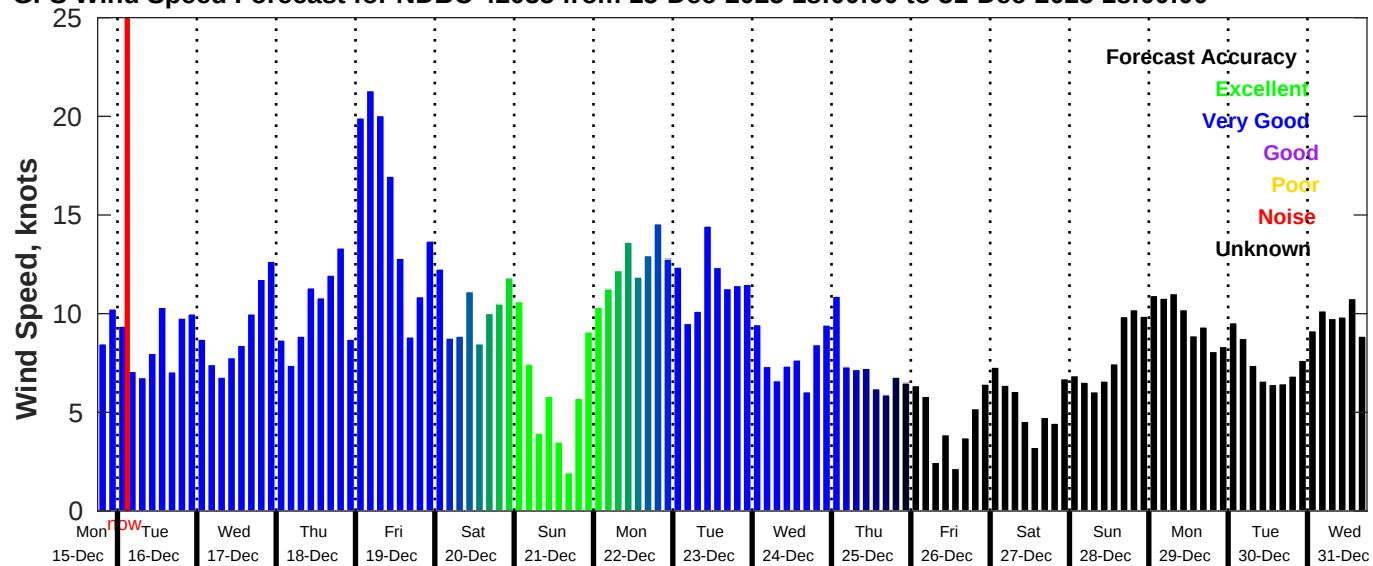
GFS Wind Speed Forecast for NDBC 42035 from 15-Dec-2025 18:00:00 to 31-Dec-2025 18:00:00
