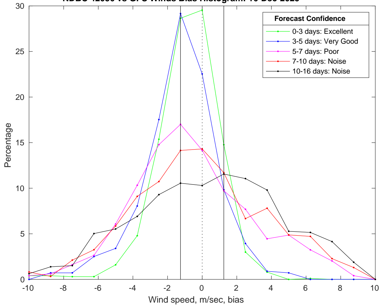
NDBC 42036 vs GFS Winds Bias Histogram: 16-Dec-2025
