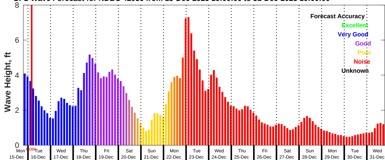
GFS Wave Forecast for NDBC 42036 from 15-Dec-2025 19:00:00 to 31-Dec-2025 19:00:00
