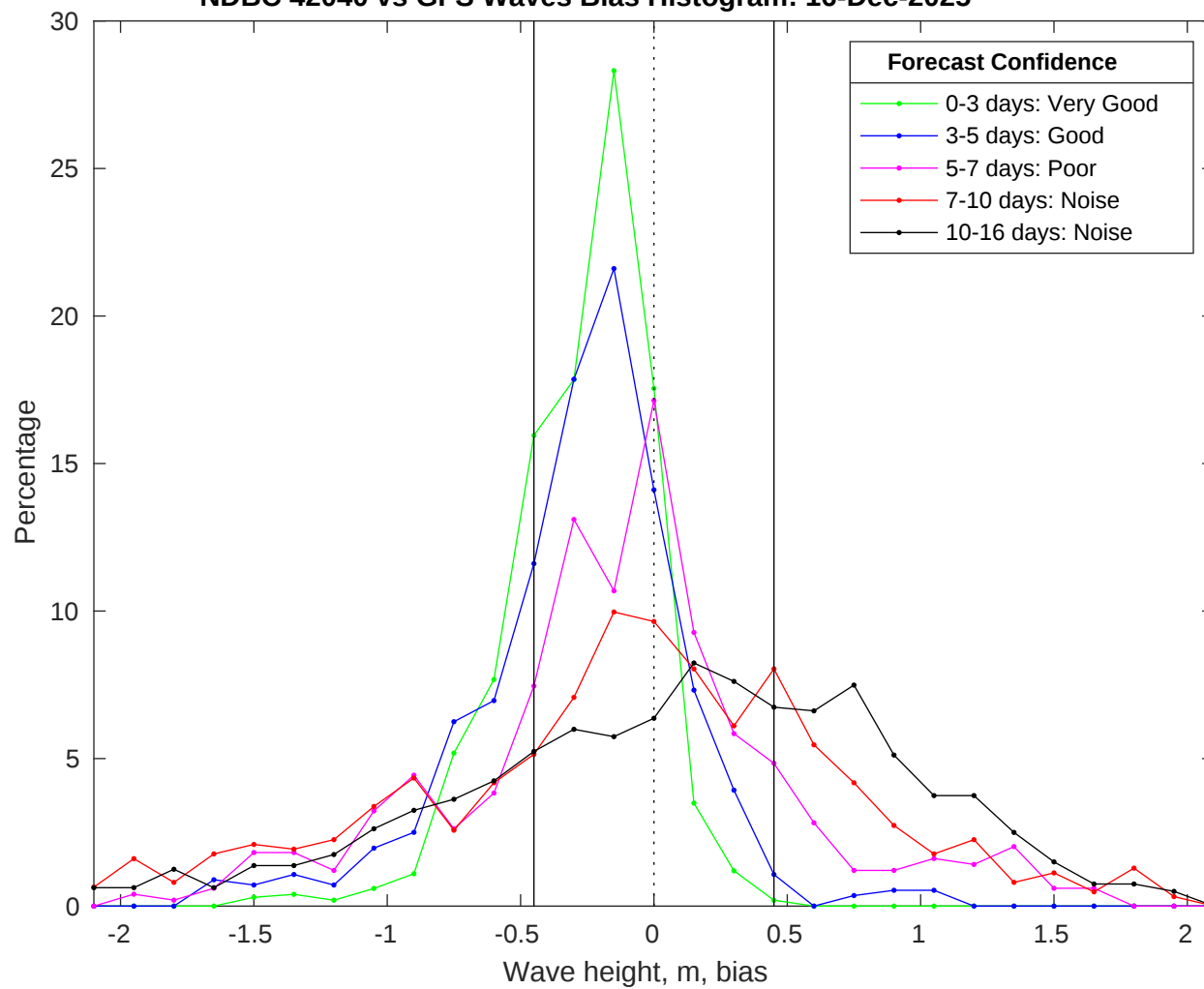
NDBC 42040 vs GFS Waves Bias Histogram: 16-Dec-2025
