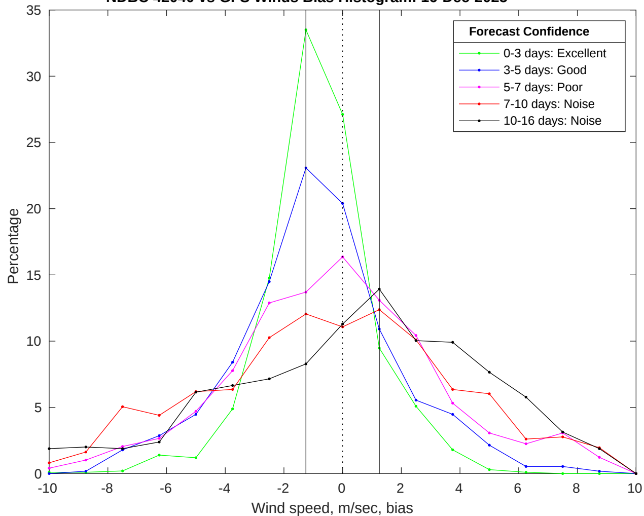
NDBC 42040 vs GFS Winds Bias Histogram: 16-Dec-2025
