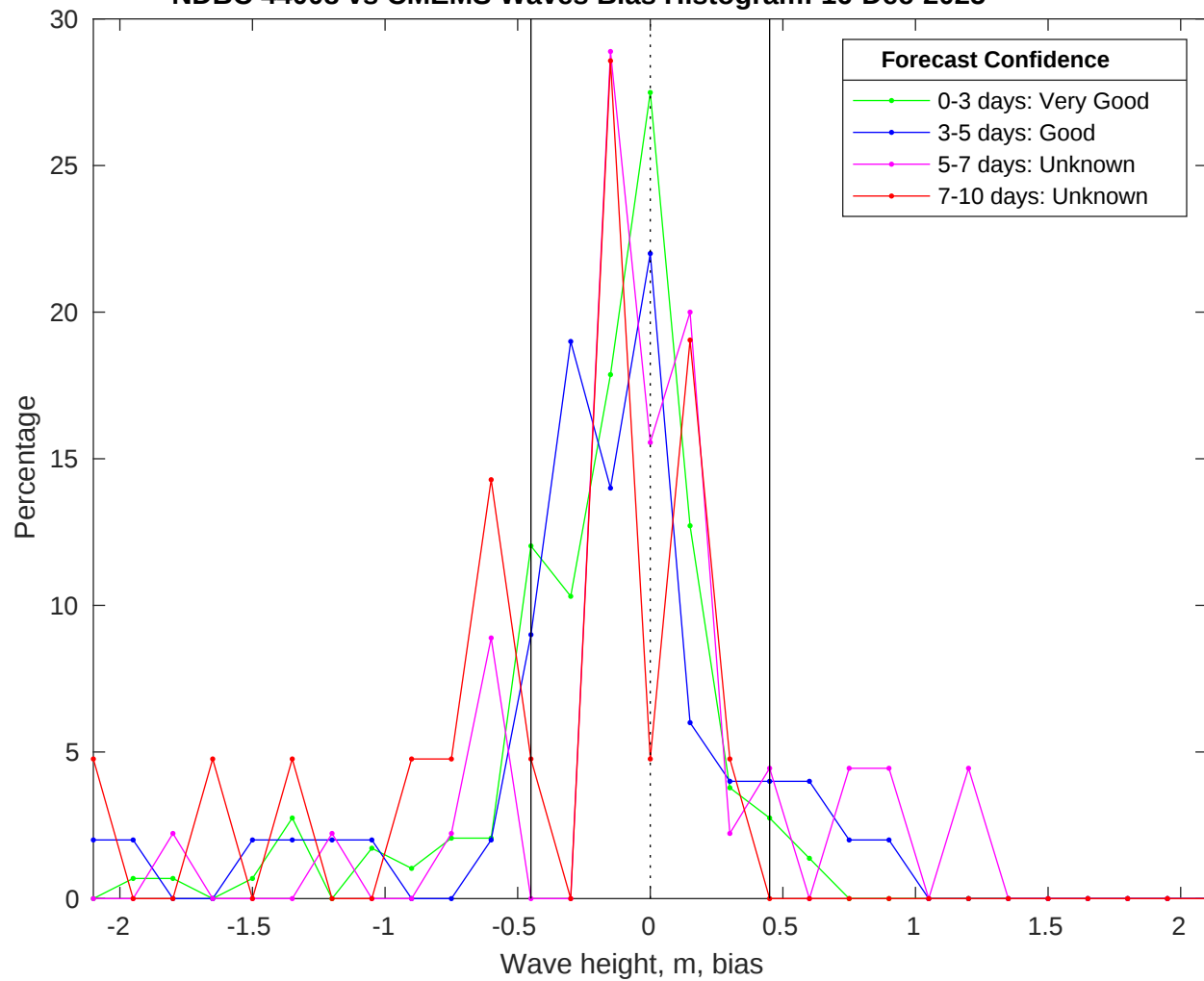
NDBC 44008 vs CMEMS Waves Bias Histogram: 16-Dec-2025
