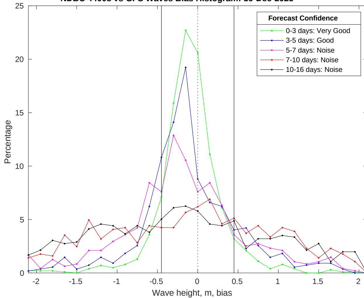
NDBC 44008 vs GFS Waves Bias Histogram: 16-Dec-2025
