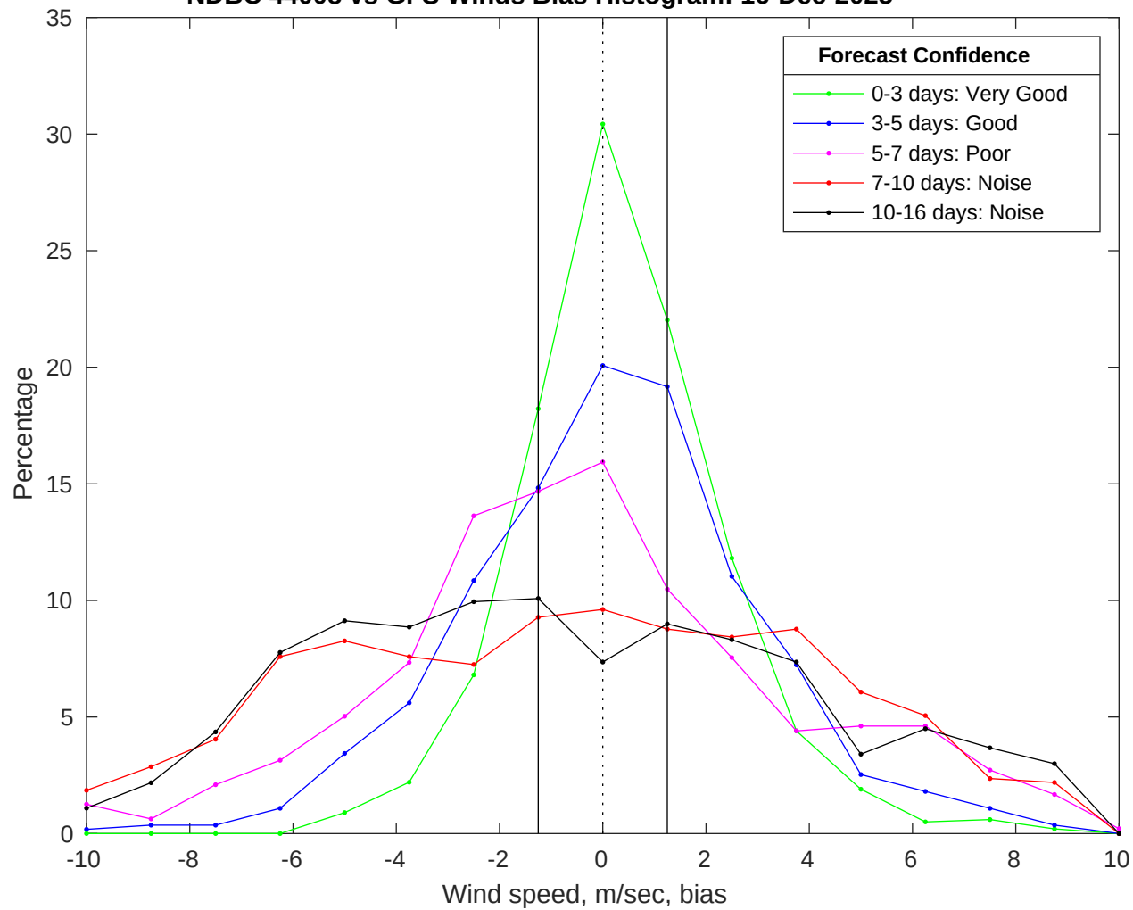
NDBC 44008 vs GFS Winds Bias Histogram: 16-Dec-2025
