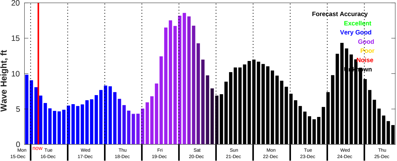
CMEMS Wave Forecast for NDBC 44008 from 15-Dec-2025 20:00:00 to 25-Dec-2025 20:00:00
