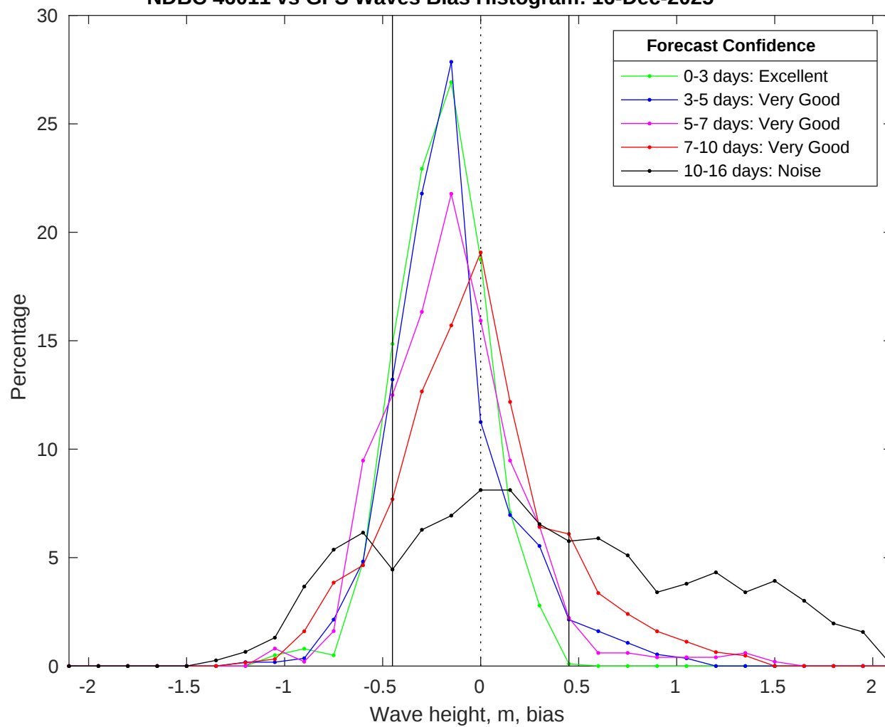
NDBC 46011 vs GFS Waves Bias Histogram: 16-Dec-2025
