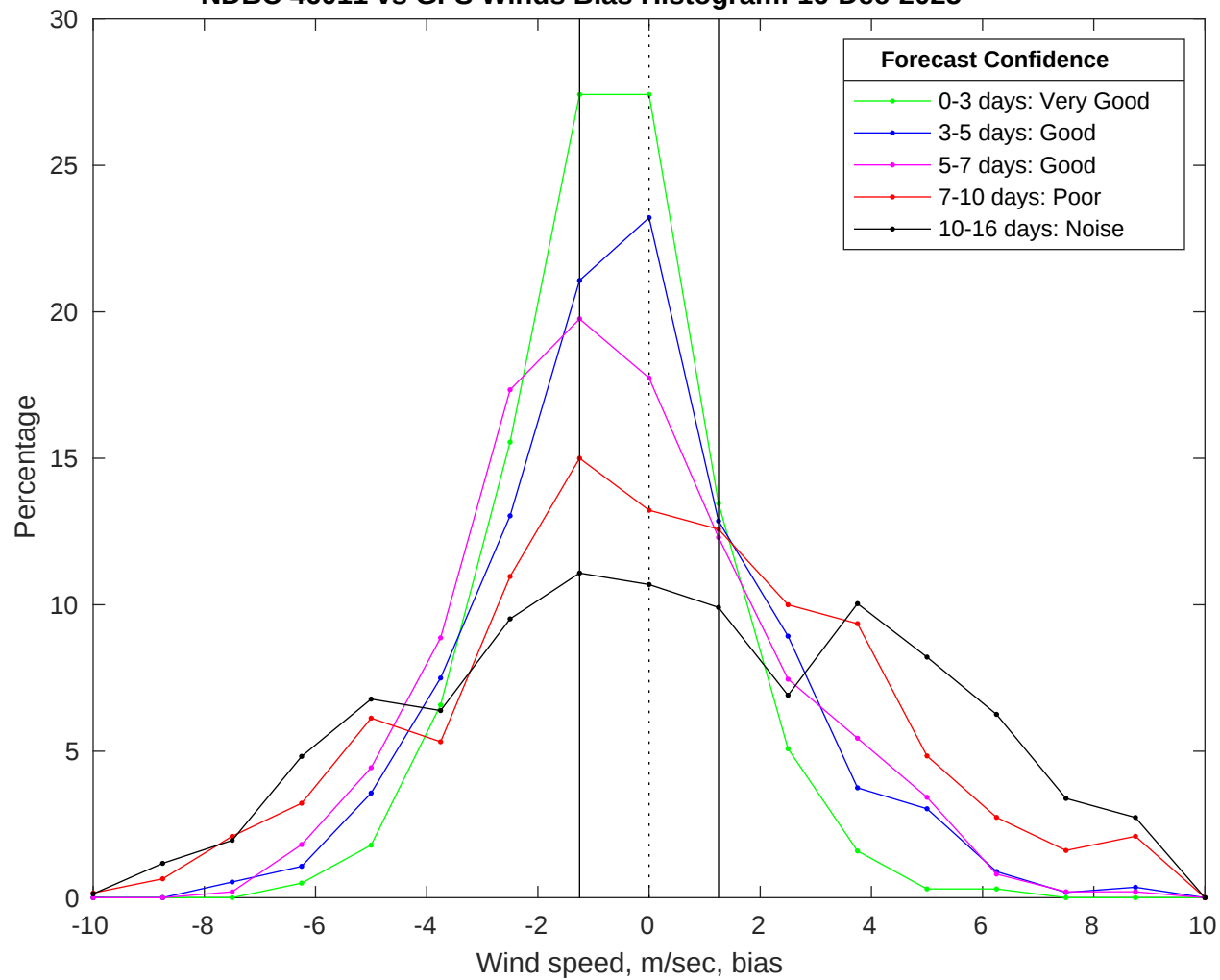
NDBC 46011 vs GFS Winds Bias Histogram: 16-Dec-2025
