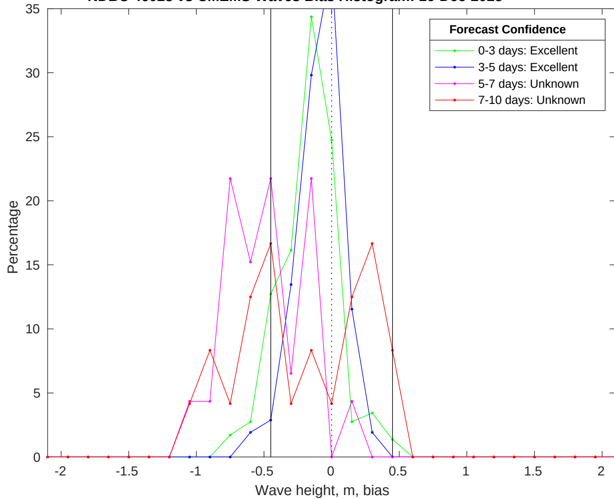
NDBC 46028 vs CMEMS Waves Bias Histogram: 16-Dec-2025
