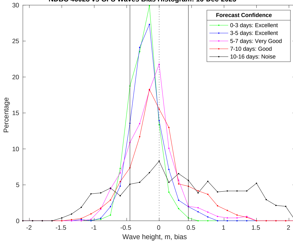
NDBC 46028 vs GFS Waves Bias Histogram: 16-Dec-2025
